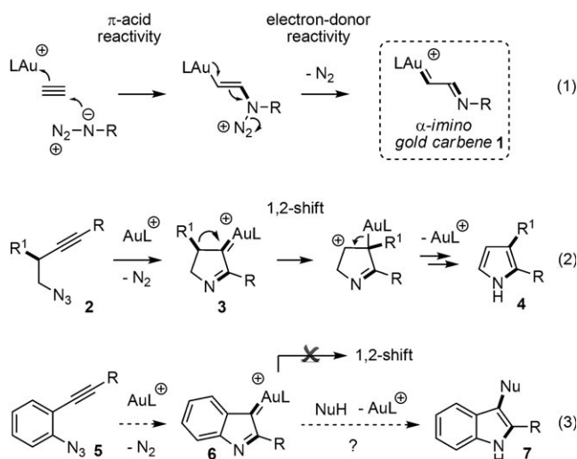
Scheme 1. Synthetic design for the trapping of \alpha -imino gold carbene. R^1 = H , alkyl, aryl.
